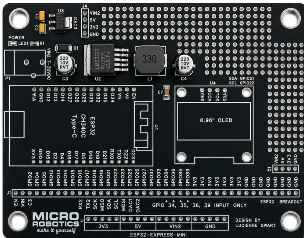
IOT Controller PC Board
